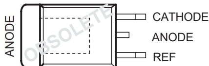
TL431 . . . KTP (PowerFLEX m /TO-252) PACKAGE (TOP VIEW)
